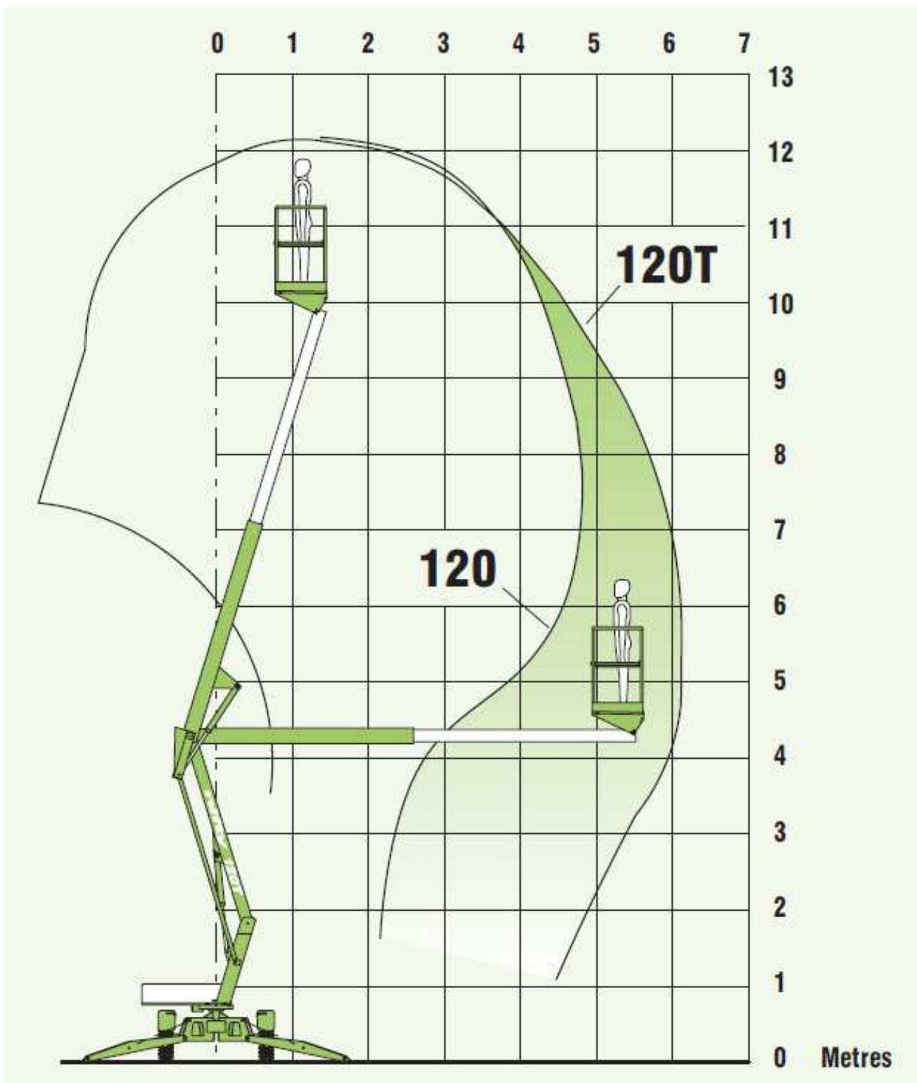
Niftylift 120T
